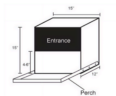
Example of a nest box design.
