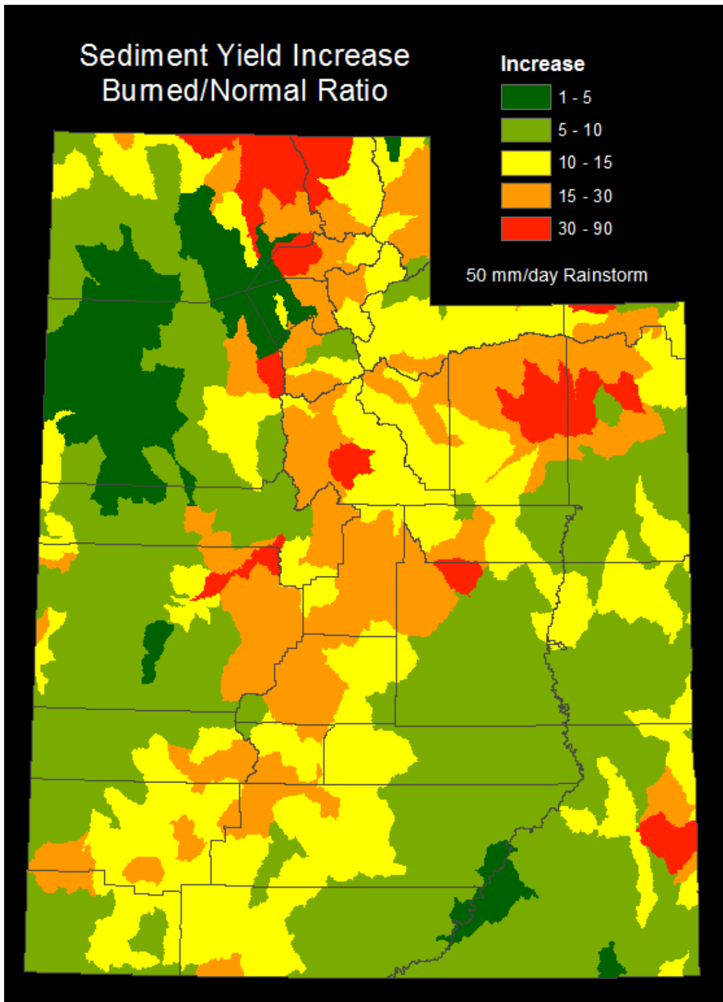
Figure 6.8: Burn /Normal ratios of sediment yields following a 50 mm storm. Results are averaged for HUC 10 watershed units within the state.
