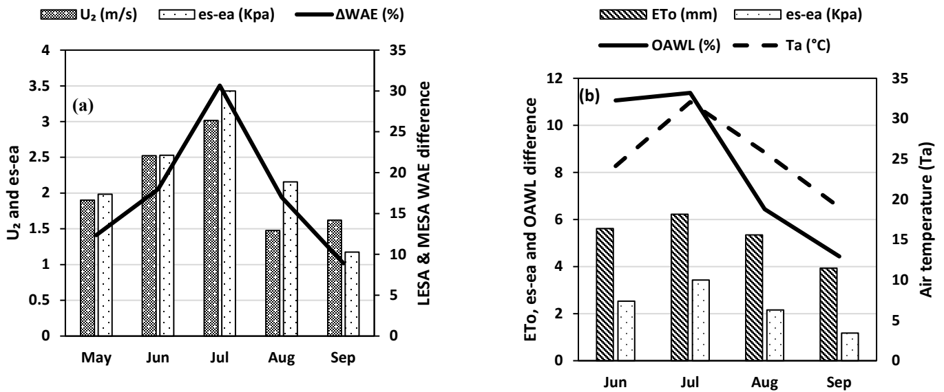
Figure 57. The mean water application efficiency differences ( \Delta WAE ) between LESA and MESA for 2015-2017 on a monthly basis along with monthly average windspeed ( U_z ) and vapor pressure deficit (air aridity, e_s - e_a )(a). The overall spray water losses (OAWL) differences between LESA and MESA for the study duration (2015-2017) on a monthly basis plotted together with reference evapotranspiration ( ET_o ), air temperature ( T_a ), and vapor pressure deficit ( e_s - e_a )(b).
