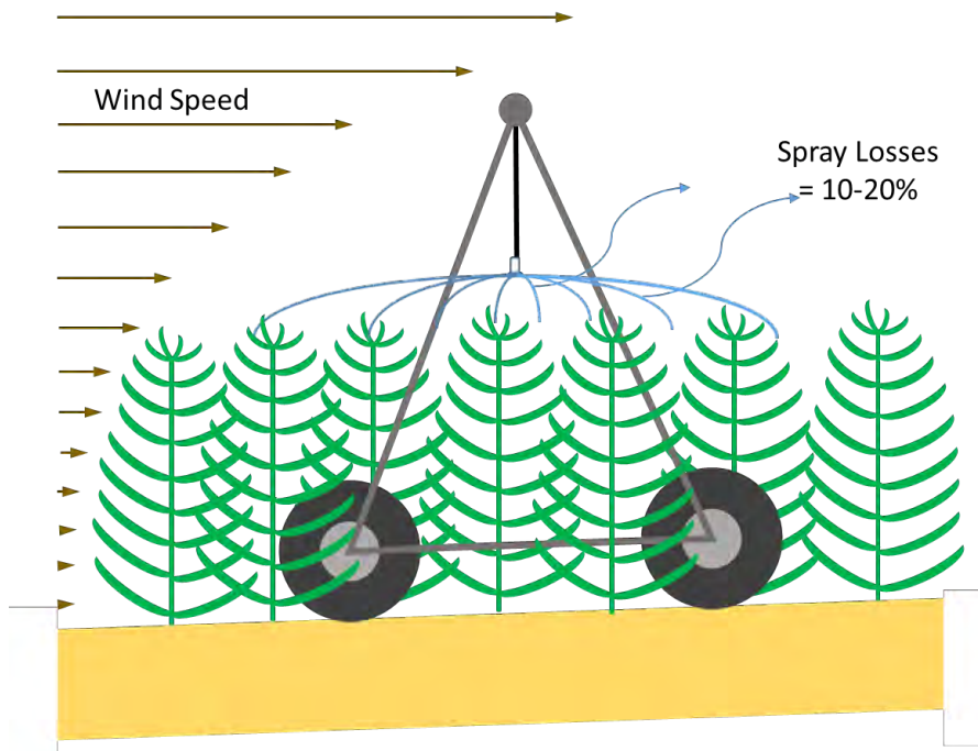
Figure 47. Moving sprinklers closer to the top of the canopy reduces spray losses to wind drift and evaporation. The typical mid-elevation spray application (MESA) sprinkler losses 10-20% of the water to wind drift and evaporation.
