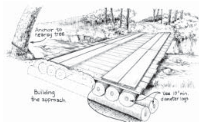
Log stringer bridge
